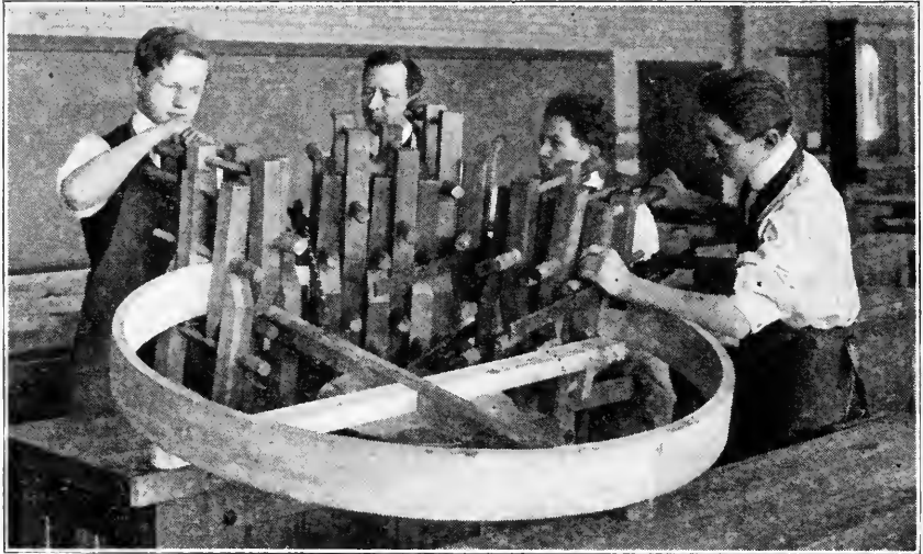
FIG. 410. APPLYING VENEER TO SEGMENTAL CORE.
